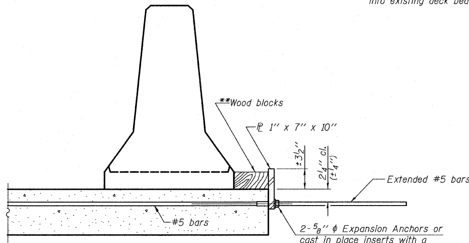
DETAIL II
