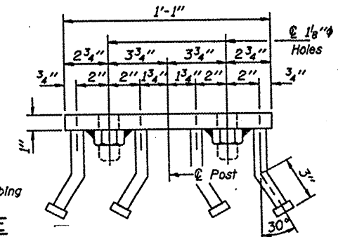
VIEW C-C
