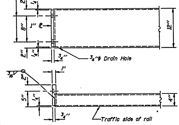
END OF RAIL DETAILS
