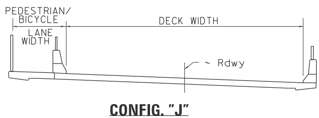
PARAPET/SAFETY WALK CONFIGURATIONS (Not To Scale)
