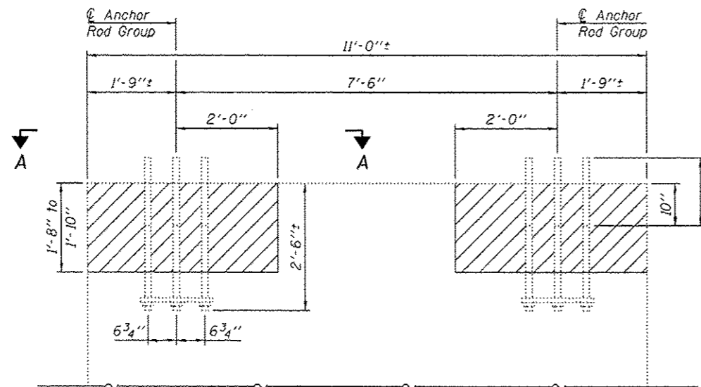
EXISTING ELEVATION OF LEFT OR RIGHT SIGN STRUCTURE FOUNDATION
