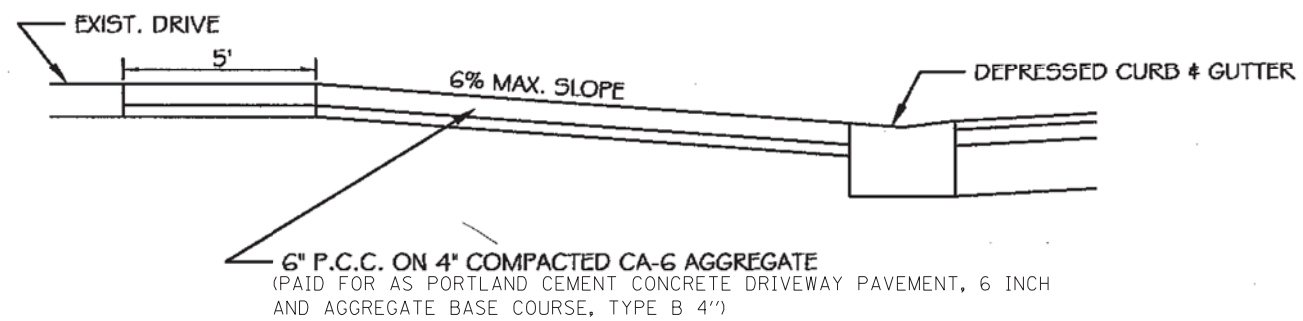
PROFILE VIEW
