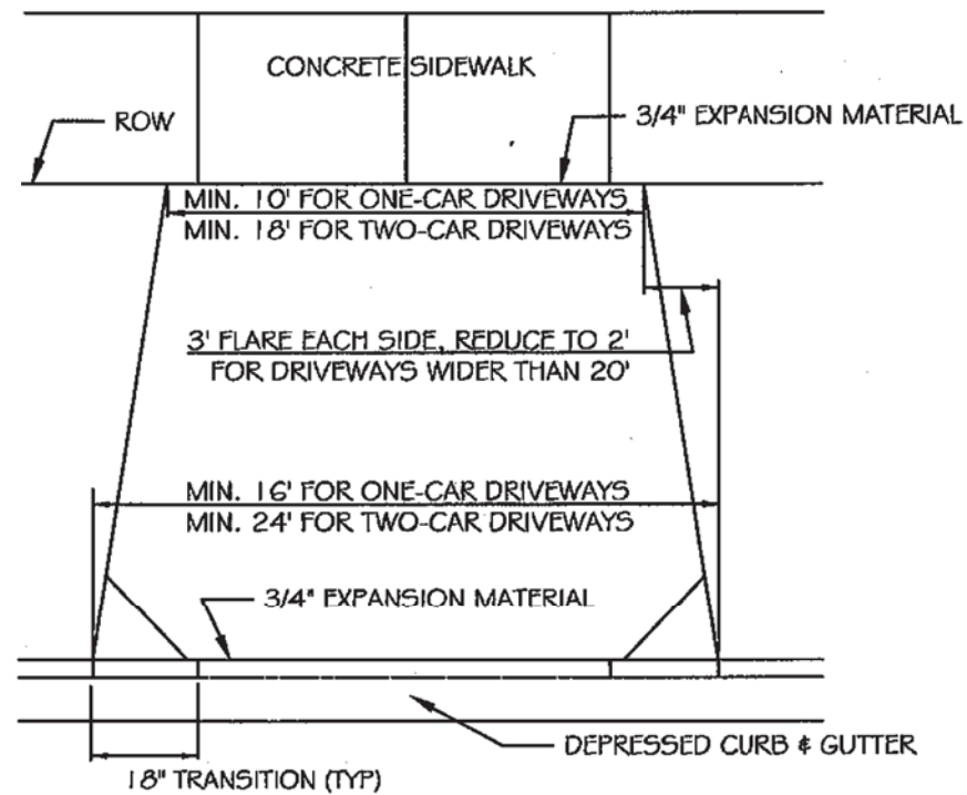
PLAN VIEW
