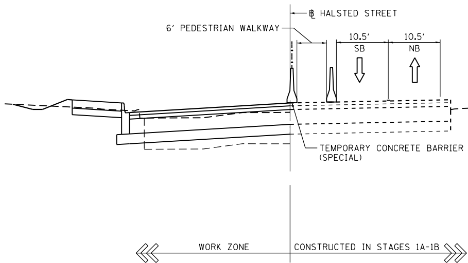
STAGE 2A AND 2B HALSTED STREET MAINTENANCE OF TRAFFIC TYPICAL SECTION
