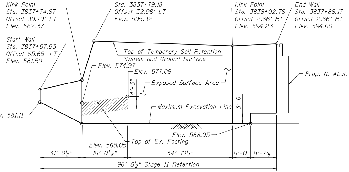
TEMPORARY SOIL RETENTION SYSTEM NO. 2 (At North Abutment)
