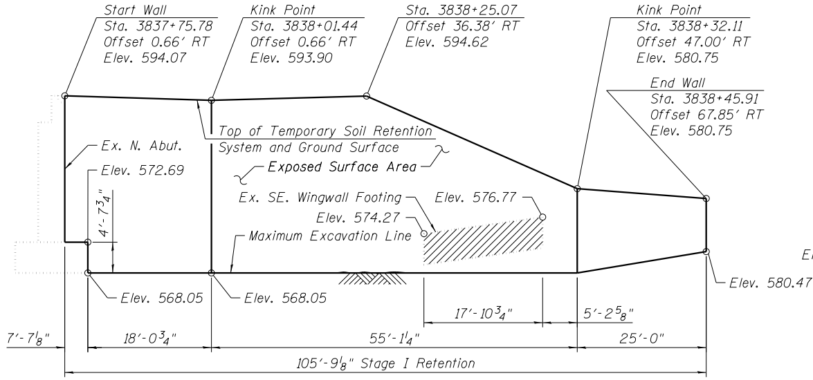
TEMPORARY SOIL RETENTION SYSTEM NO. 1 (At North Abutment)
