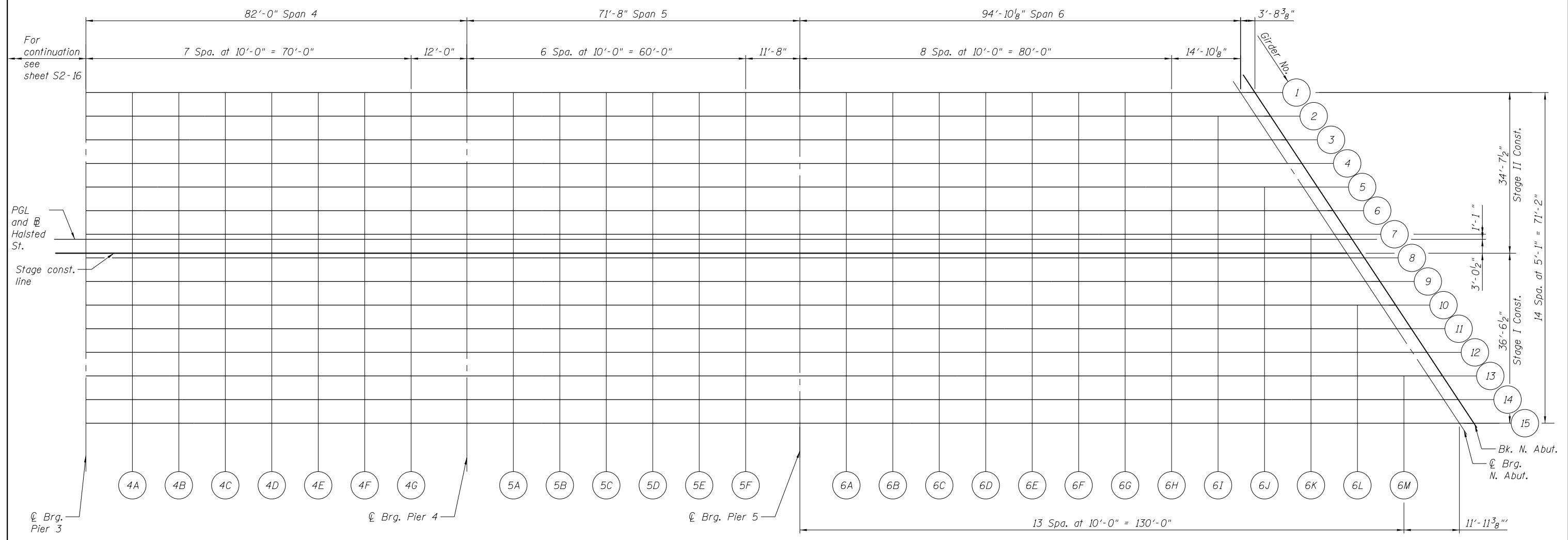
PLAN (Spans 4, 5 and 6)
