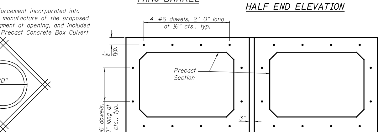
PRECAST CONCRETE CULVERT END ELEVATION (Section is symmetrical about centerline of culvert)
