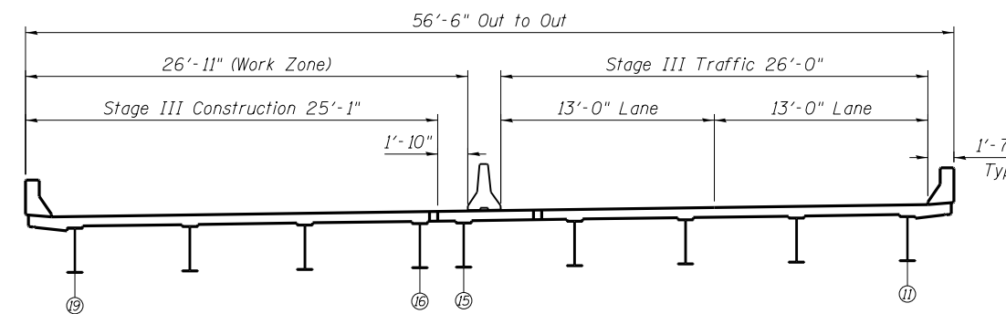
SN 082-0153 WESTBOUND CROSS SECTION
