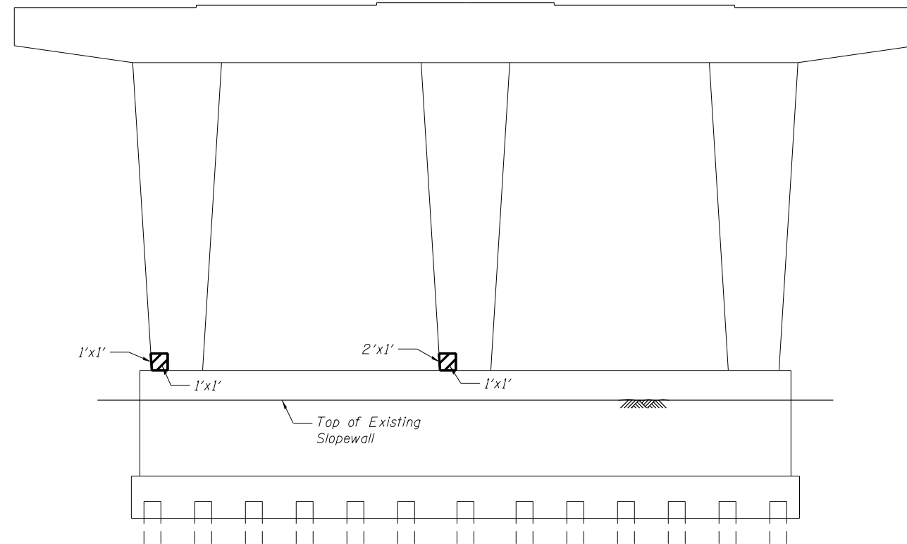
STRUCTURE 082-0157 EAST PIER (Looking East)
