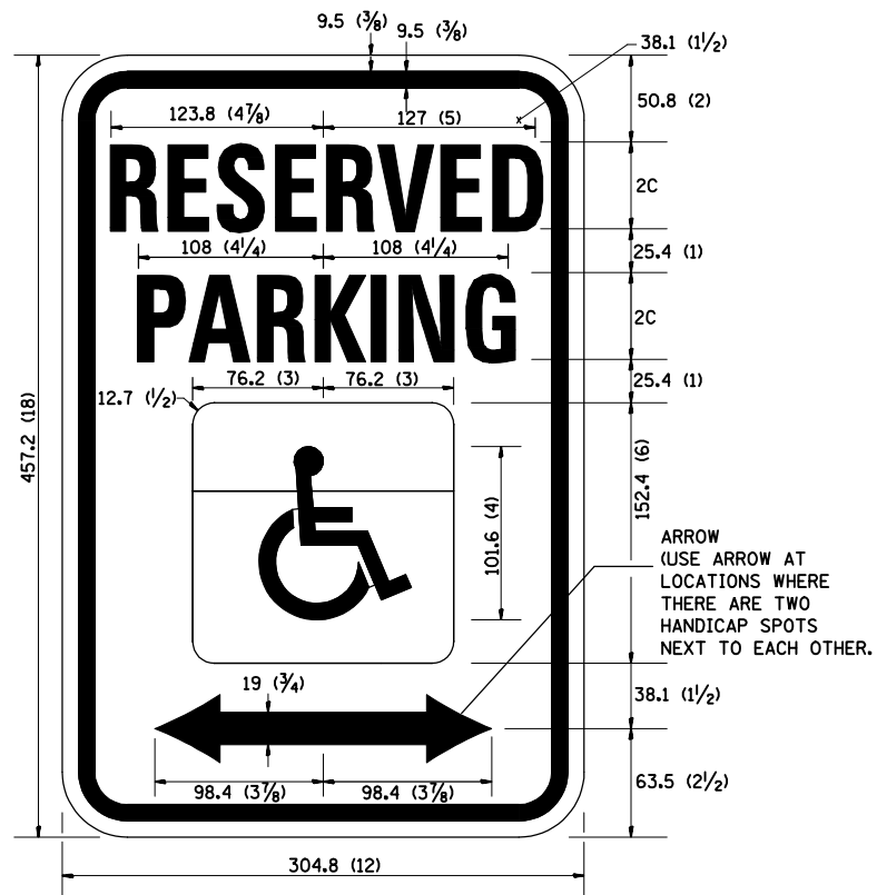
SIGN R7-8
