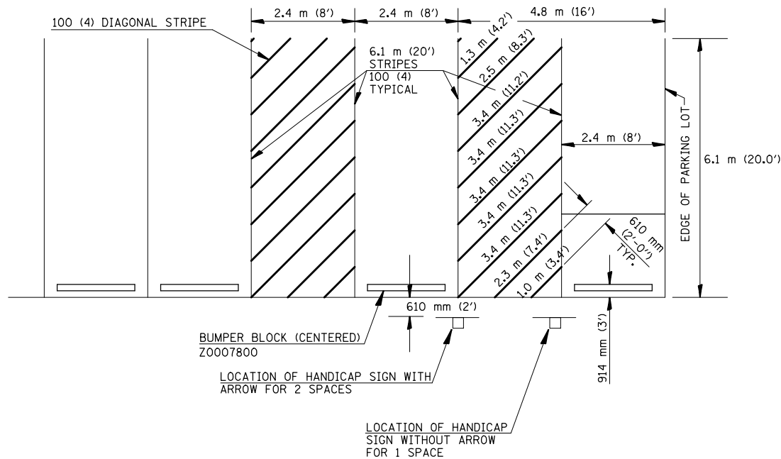
DETAIL OF PARKING SPACES
