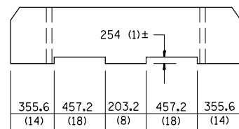
ELEVATION VIEW
