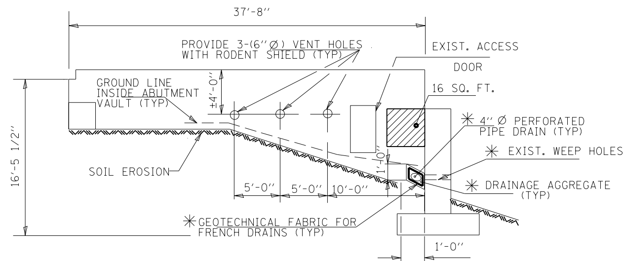
WEST ABUTMENT CURTAIN WALL LOOKING NORTH
