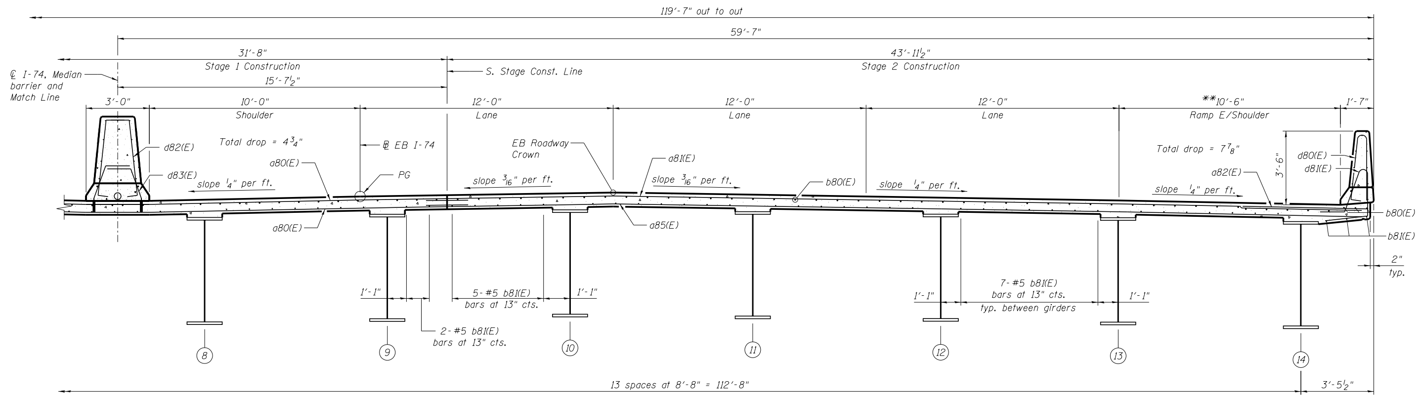
CROSS SECTION (Looking Upstation)
