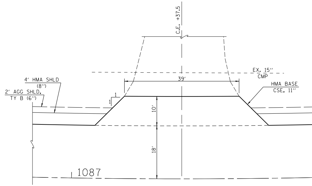
DETAIL (C.E. 1087+37.5)
