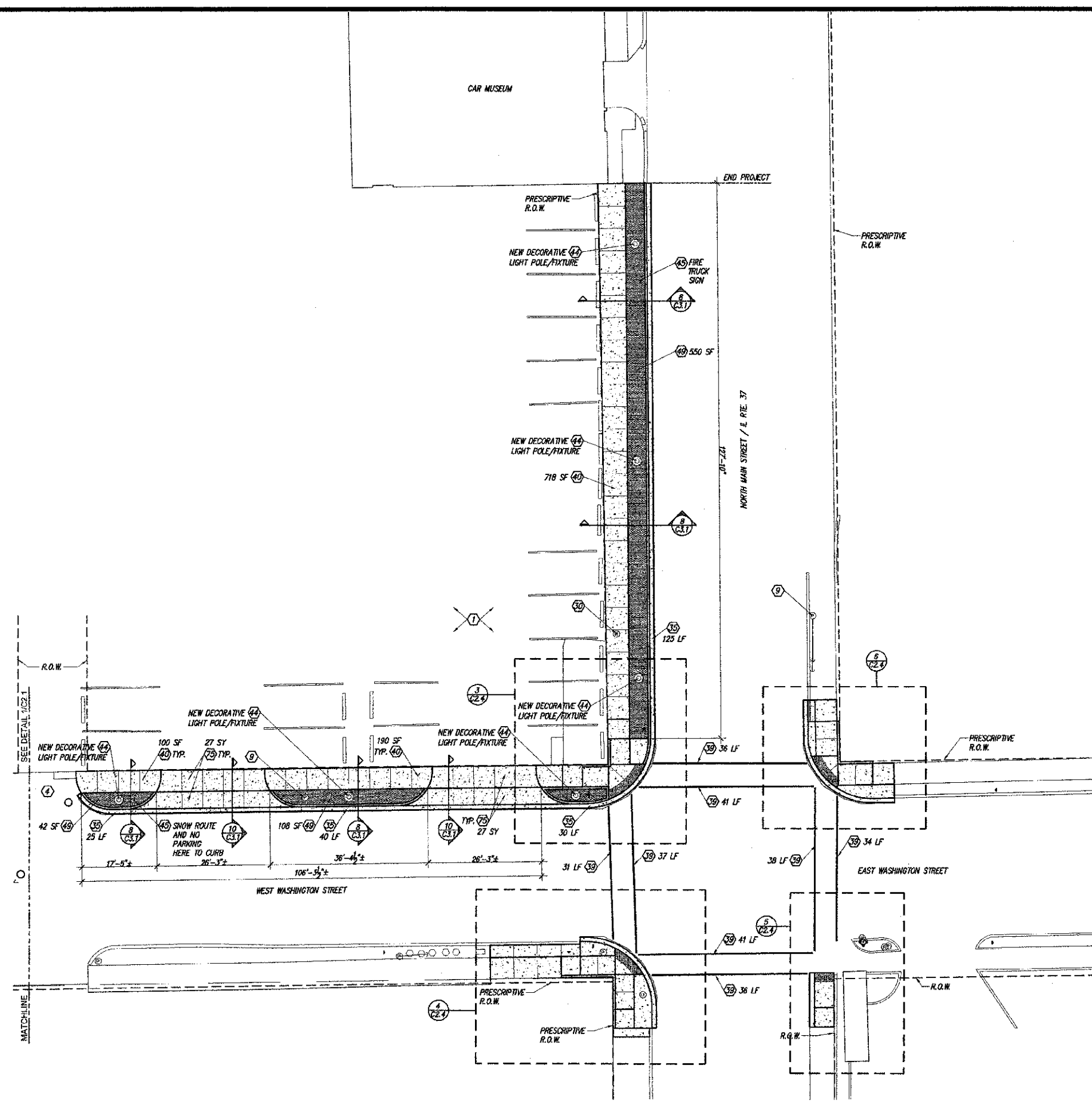
1 LARGE SCALE SITE LAYOUT PLAN - WASHINGTON AND NORTH MAIN STREETS SCALE: 1/16"=1'-0"
