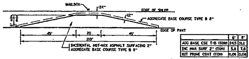
HOT-MIX ASPHALT APPROACHES & MAILBOX RETURNS FOR TWO LIFT (3P) RESURFACING PROJECTS 41.2 REVISED 10-10-06
