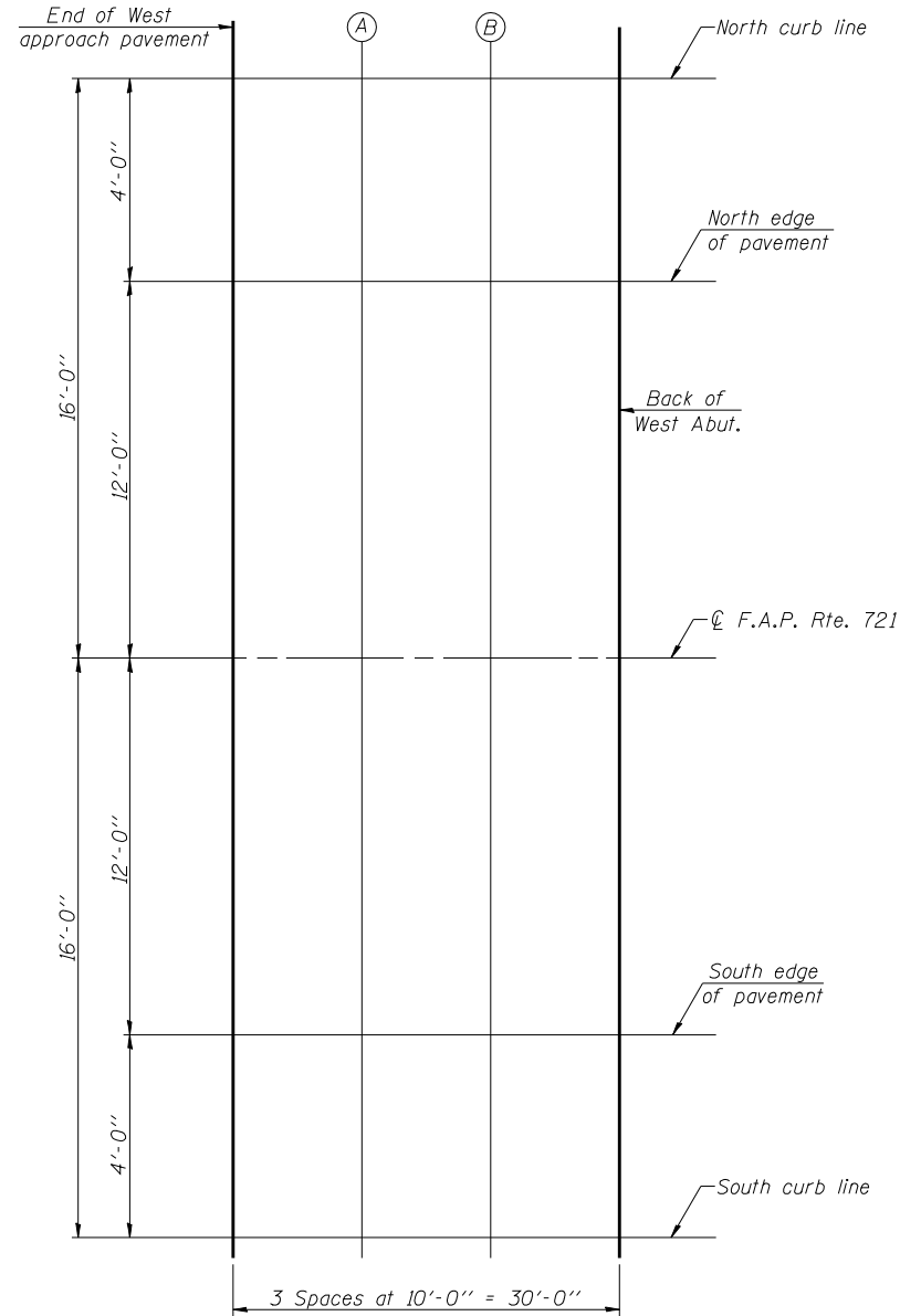
PLAN
