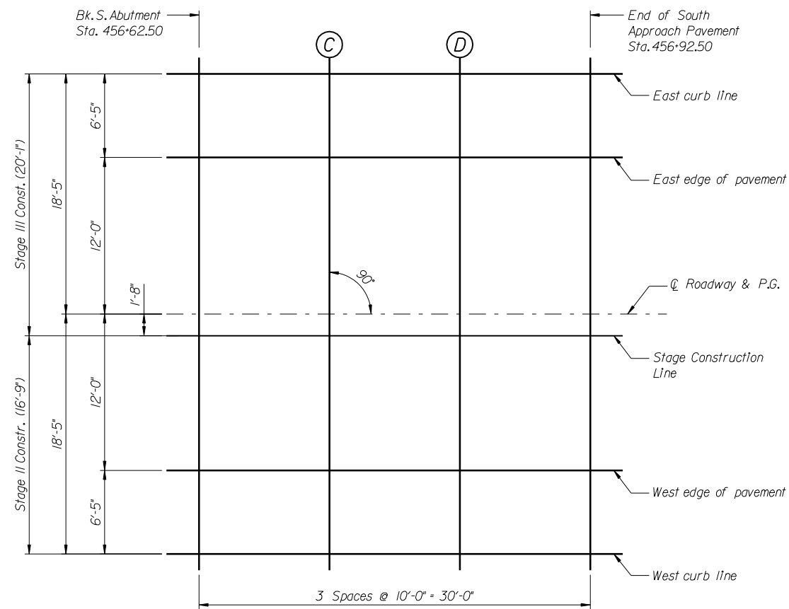
PLAN - SOUTH APPROACH PAVEMENT
