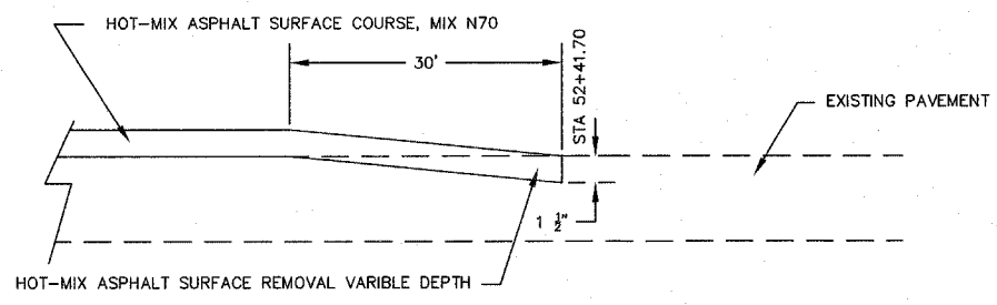
BUTTJOINT DETAIL
