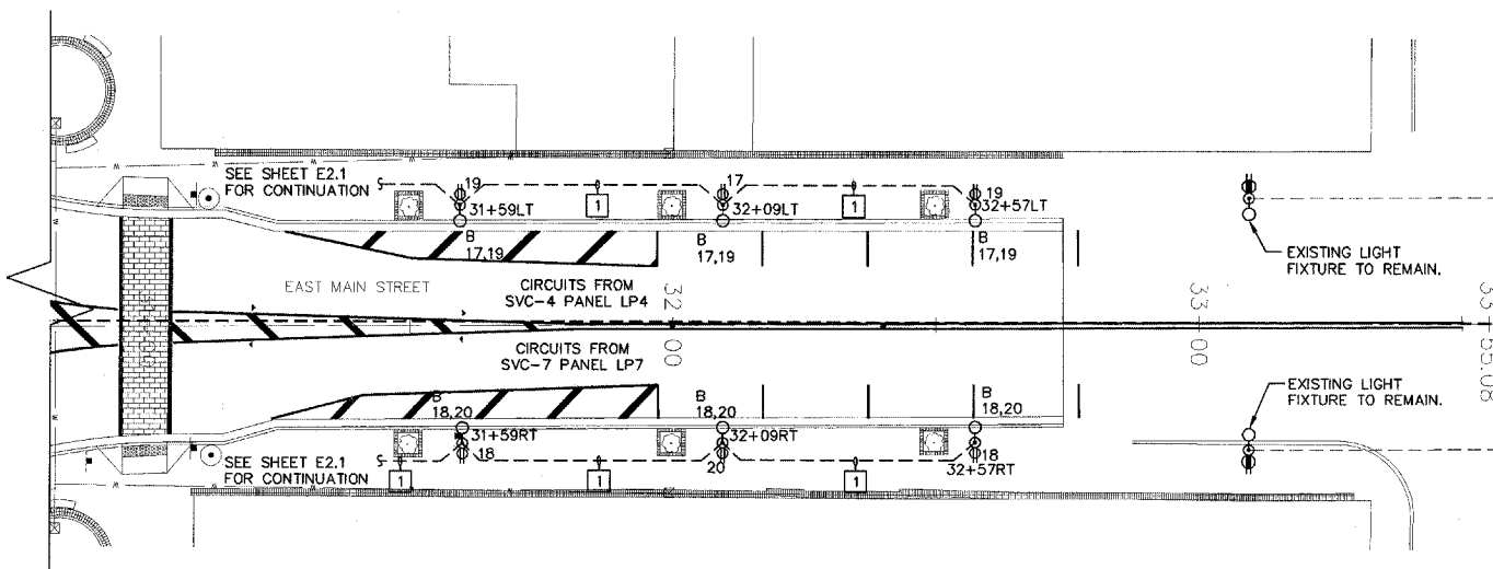
EAST ELECTRICAL PLAN - LIGHTING 1" = 20'-0"
