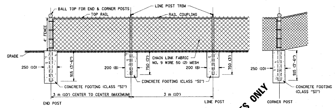
CHAIN LINK FENCE
