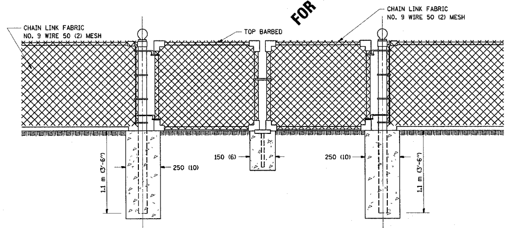
DRIVE GATE 1 m (3'-7") X 3 m (10')
