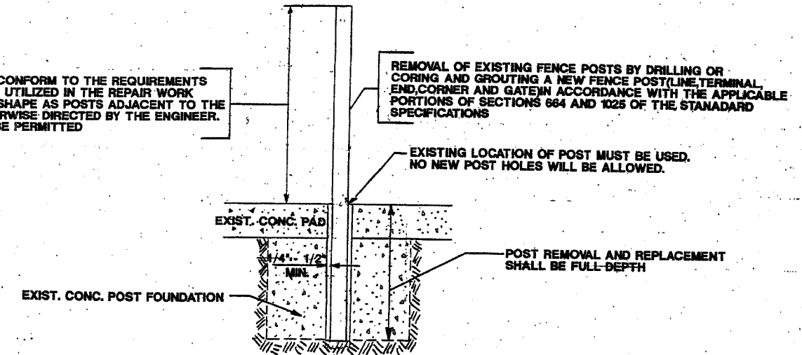
POST REMOVAL AND REPLACEMENT
