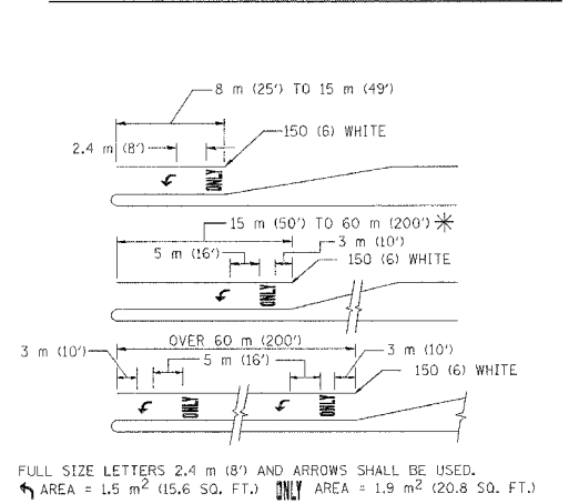
TYPICAL PAINTED MEDIAN MARKING
