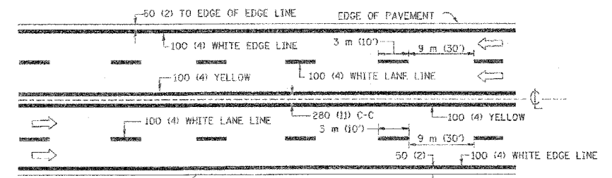
MULTI-LANE UNDIVIDED
