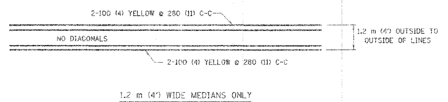
1.2 m (4') WIDE MEDIANS ONLY
