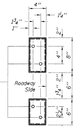
END OF RAIL DETAILS
