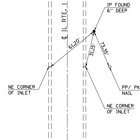
TS 9212 214+35.63, 33.43' RT.
