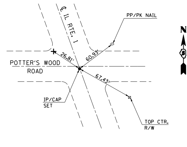
PI #4 218+64.68
