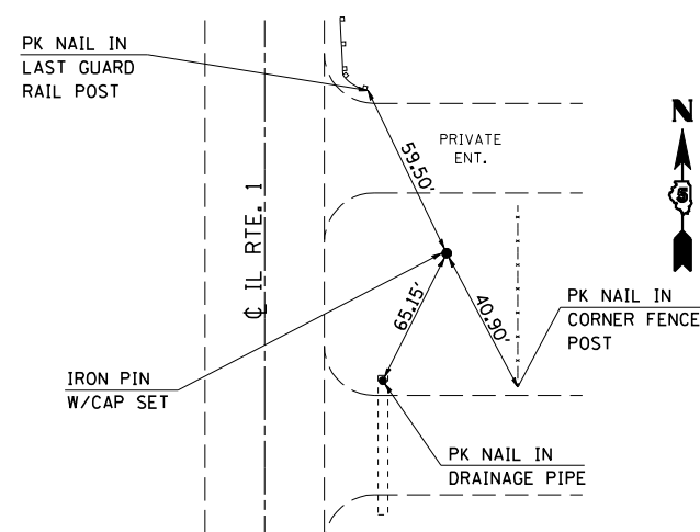
TS 400 195+18.12, 36.16' RT.
