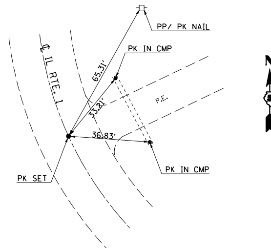
PT 194+47.71 #16
