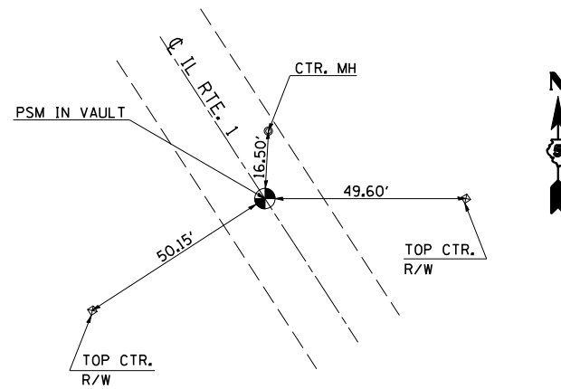
PT 194+47.71 #16
