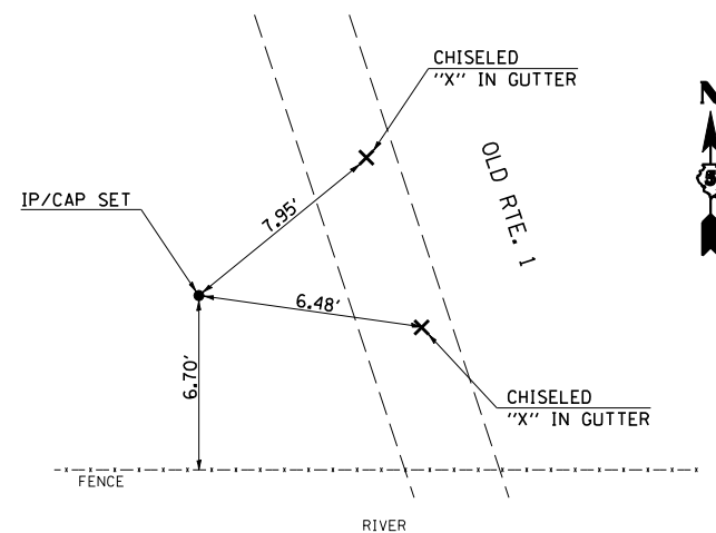
TS 401 200+61.43, 453.72' LT.
