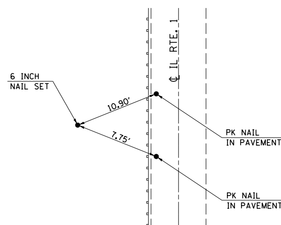
TS 402 201+55.53, 24.79' LT.
