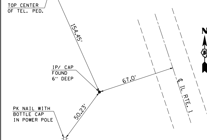
TS 9211 199+66.33, 14.01' RT.
