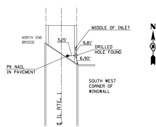
TS 9211 199+66.33, 14.01' RT.
