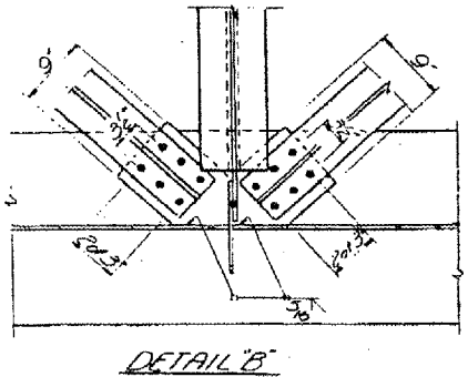
TYP LATERAL BRACE Bottom Laterals shown - Top similar
