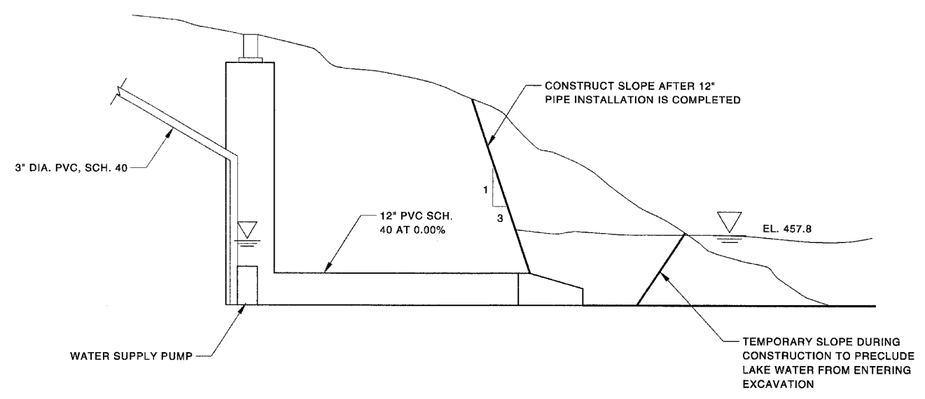
INTAKE FOR WATER SUPPLY PUMP NTS
