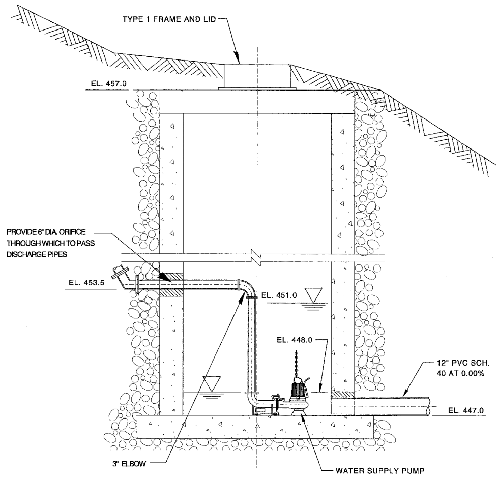
WATER SUPPLY PUMP CHAMBER NTS
