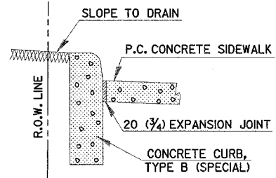
SECTION C-C CURB DETAIL ADJACENT TO EARTHFILL
