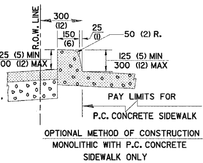
SECTION C-C CURB DETAIL ADJACENT TO EXISTING OR RECONSTRUCTED PARKING LOTS
