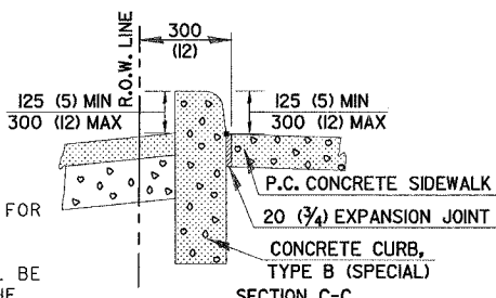
SECTION C-C CURB DETAIL ADJACENT TO EXISTING OR RECONSTRUCTED PARKING LOTS
