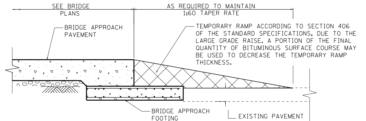
TEMPORARY RAMP TAPER DETAIL
