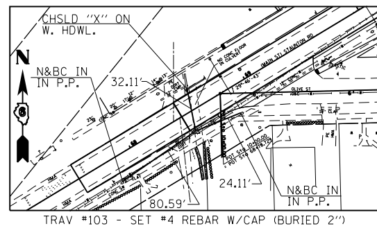
TRAV #103 - SET #4 REBAR W/CAP (BURIED 2")
