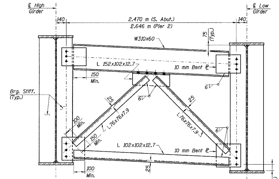
END CROSS FRAME (At South Abutment and Pier 2) (All Materials AASHTO M270M Grade 345, N.T.R.)
