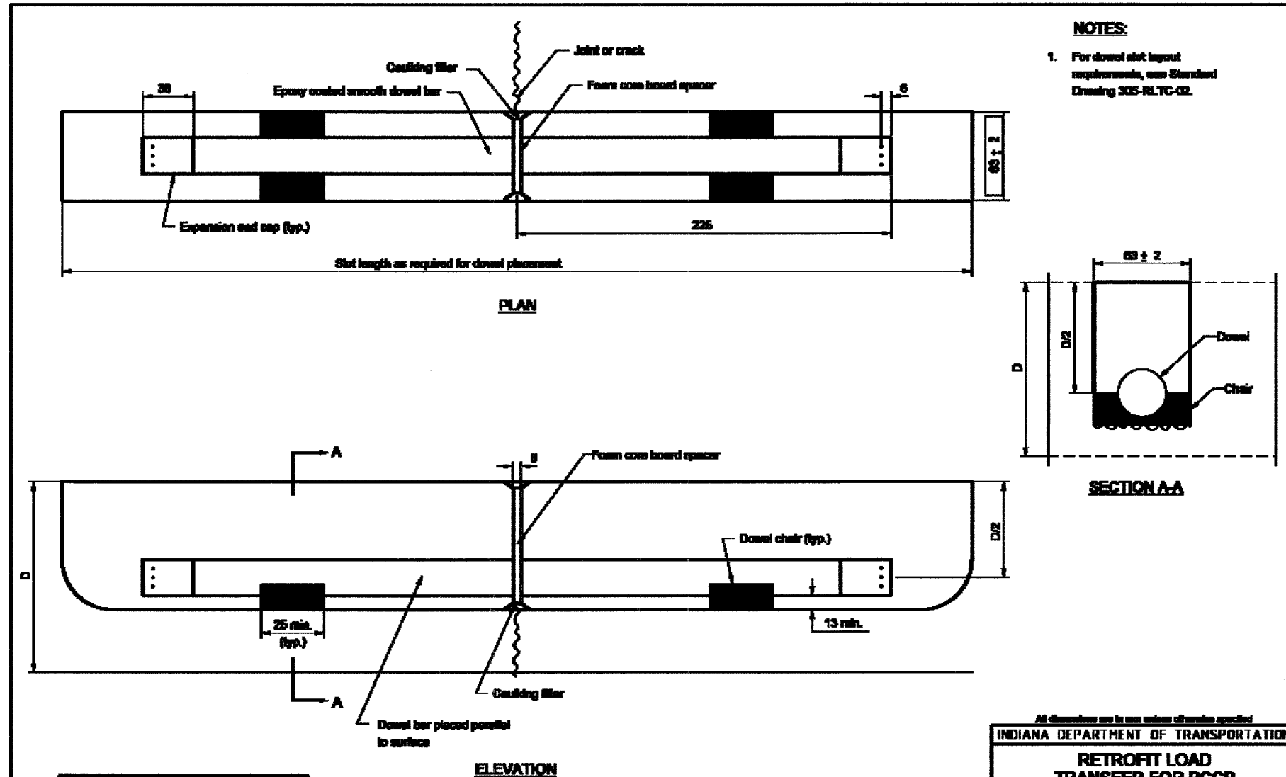
DOWEL SLOT DETAILS
