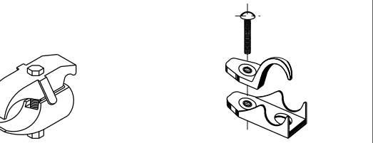
PVC COATED CONDUIT BEAM CLAMP NOT TO SCALE PVC COATED CONDUIT CLAMP NOT TO SCALE
