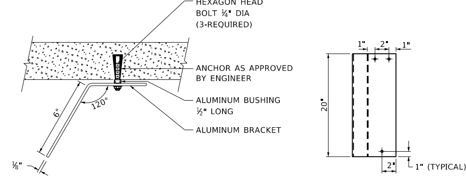
TOP VIEW ELEVATION LUMINAIRE NUMBERING DECAL BRACKET NOT TO SCALE
