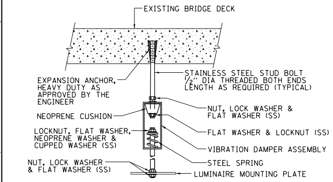
EXISTING BRIDGE DECK INSTALLATION NEW BRIDGE DECK INSTALLATION TYPICAL LUMINAIRE HANGER ASSEMBLY DETAILS
