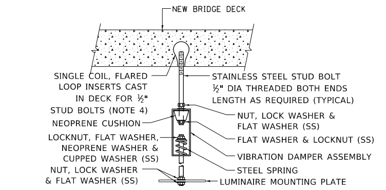
EXISTING BRIDGE DECK INSTALLATION NEW BRIDGE DECK INSTALLATION TYPICAL LUMINAIRE HANGER ASSEMBLY DETAILS
