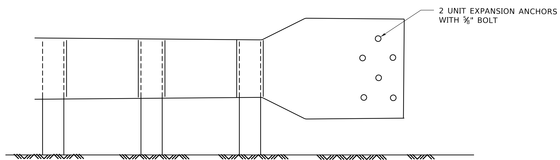
TYPICAL INSTALLATION DETAIL OF CONNECTION OF GUARDRAIL TO SQUARE BRIDGE PIER OR FOUNDATION.
