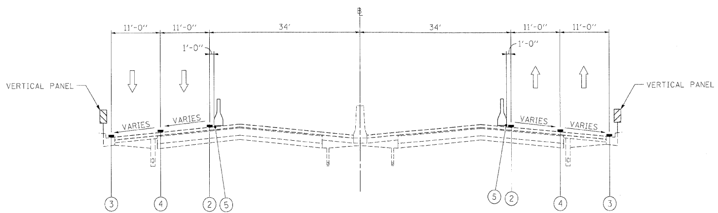
WESTBOUND MAINTENANCE OF TRAFFIC EASTBOUND TYPICAL SECTION STAGE 2 STA 503+43 TO 530+10 BRIDGE OMISSION STA 505+97 TO 526+15 STA 506+97 TO STA 509+30 STA 524+98 TO STA 525+90
