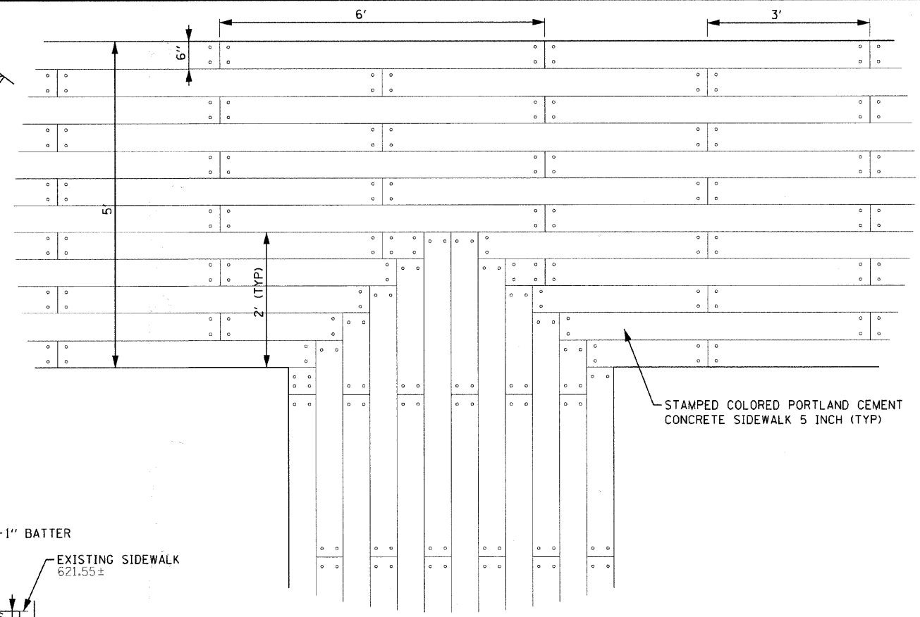
STAMPED COLORED PORTLAND CEMENT CONCRETE SIDEWALK AT STREET LIGHT DETAIL (NOT TO SCALE)
