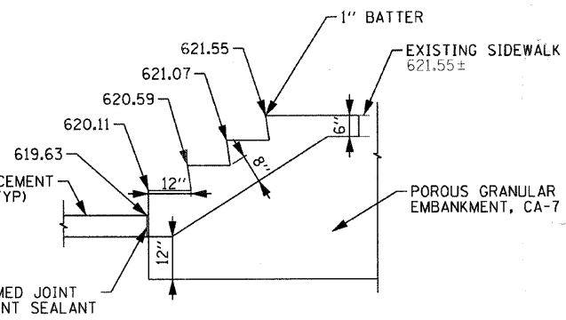
STAMPED COLORED PORTLAND CEMENT CONCRETE SIDEWALK AT STREET LIGHT DETAIL (NOT TO SCALE)
