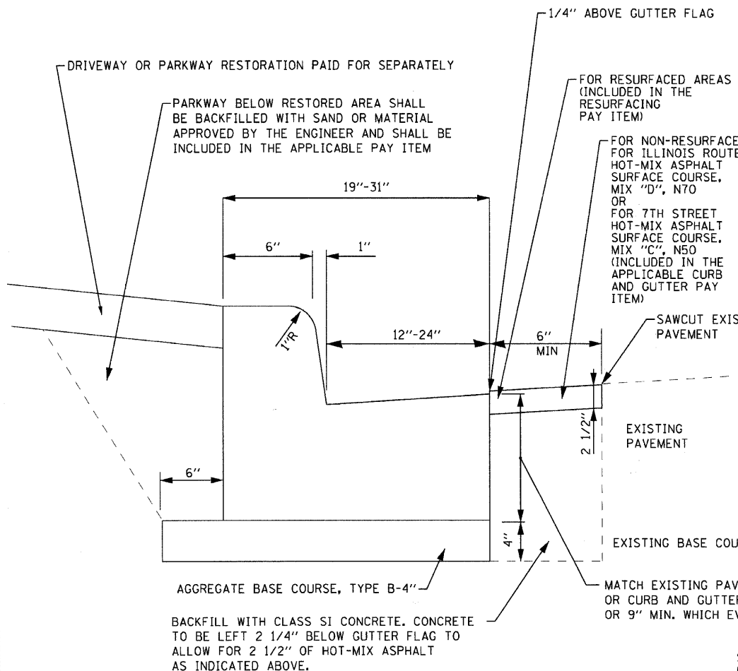
COMBINATION CURB AND GUTTER REMOVAL, COMBINATION CONCRETE CURB AND GUTTER REMOVAL AND REPLACEMENT (SPECIAL), COMBINATION CONCRETE CURB AND GUTTER TYPE B-6.12 (SPECIAL) DETAIL (NOT TO SCALE)
