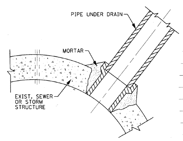
STORM SEWER CONNECTION, SPECIAL (NOT TO SCALE)
