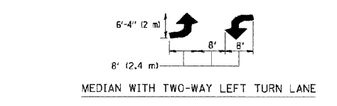
TYPICAL PAINTED MEDIAN MARKING
