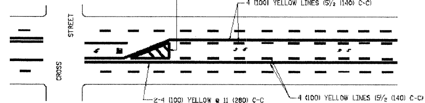
TYPICAL PAINTED MEDIAN MARKING
