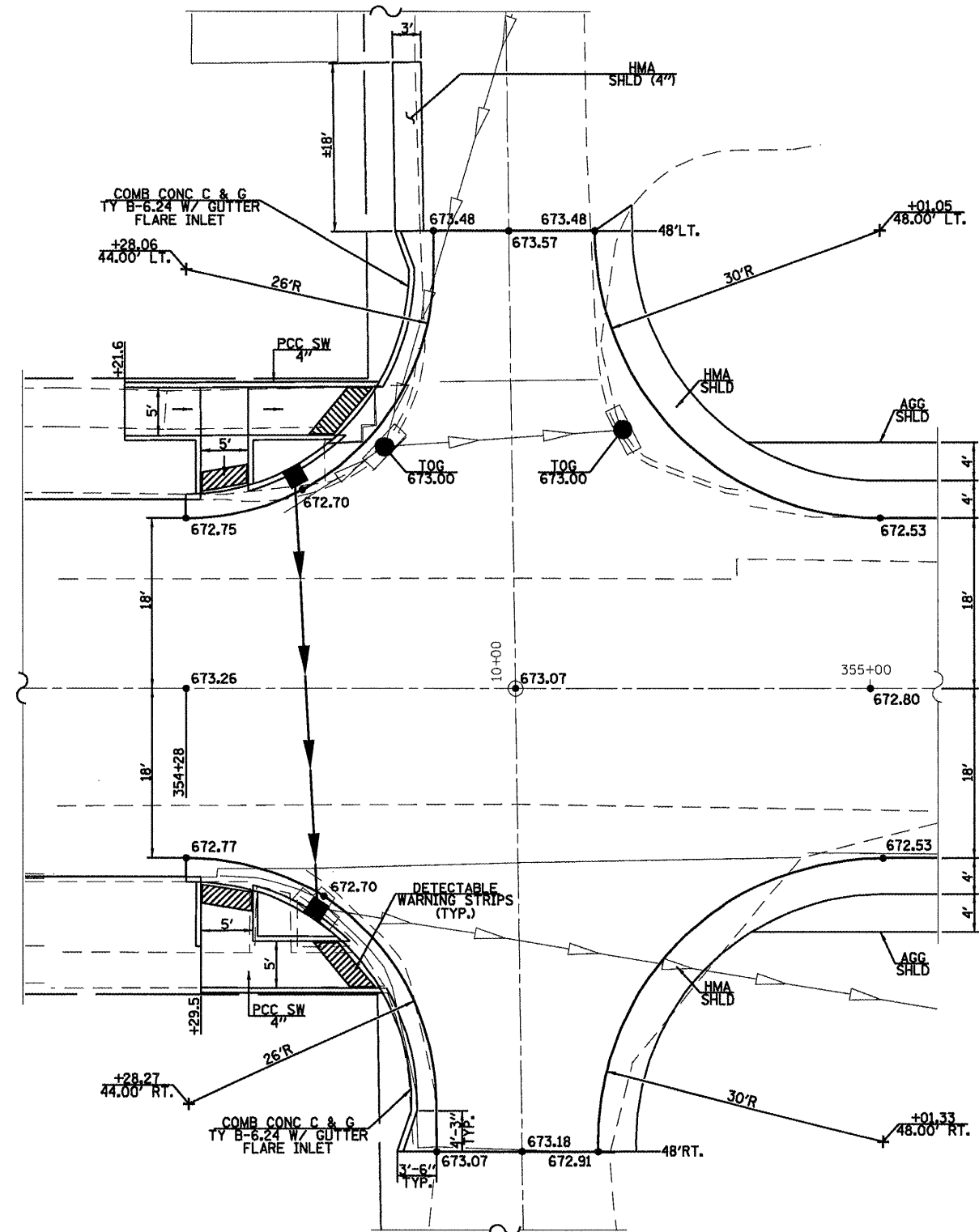
INTERSECTION DETAIL (GEORGE ST. & IL. 4)
