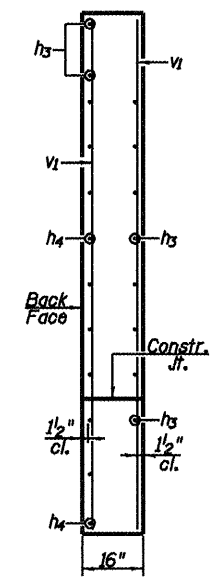
SECTION B-B
