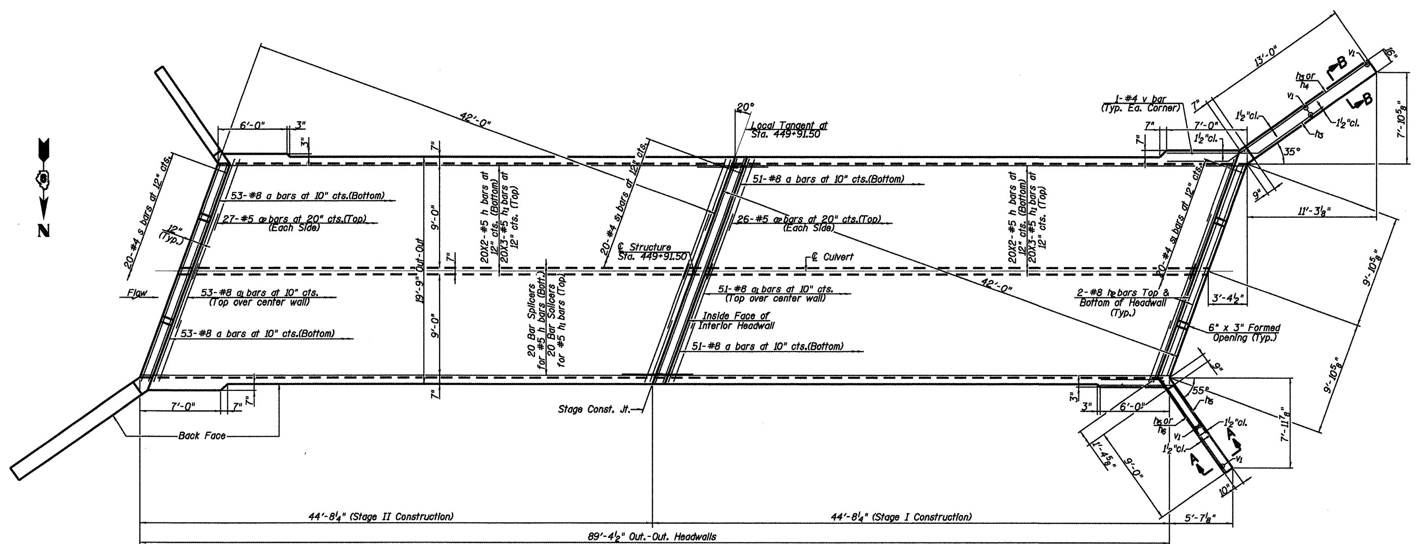
PLAN - TOP SLAB
