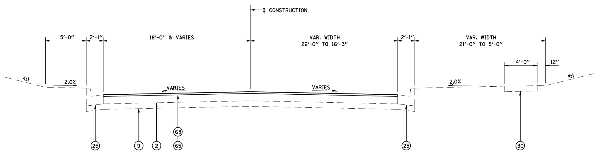
TYPICAL CROSS SECTION KOKE MILL RD STA 110+71.79 TO STA 111+51.50
