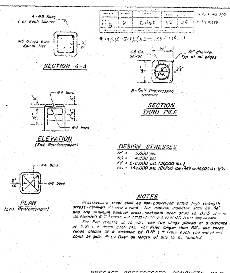
PRECAST PRESTRESSED CONCRETE PILE
