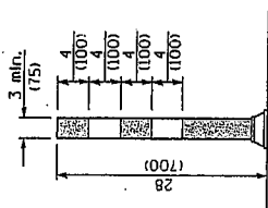
FLEXIBLE DELINEATOR
