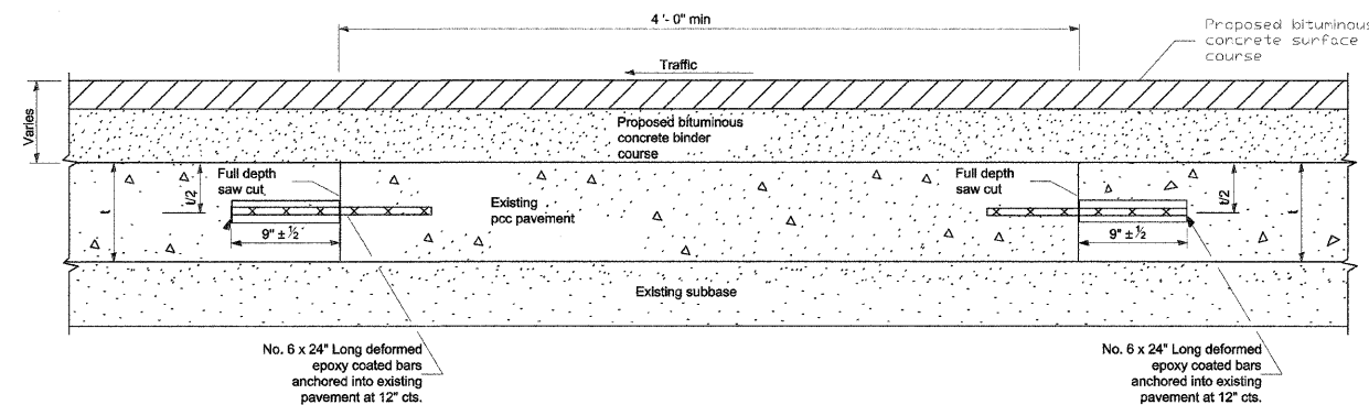
METHOD II (WITH RESURFACING)
