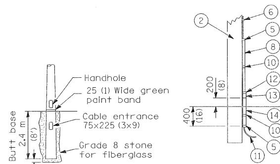
POLE, WOOD
