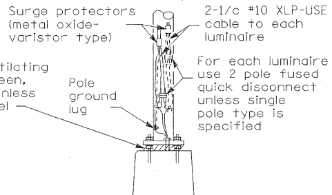
ANCHOR
