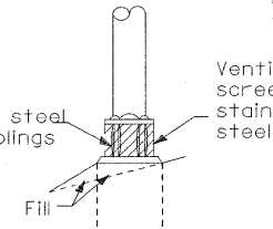
BREAKAWAY COUPLING
