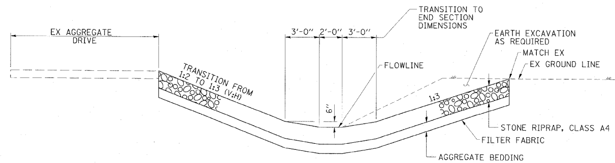
TYPICAL SECTION THRU RIPRAP LOOKING DOWNSTREAM
