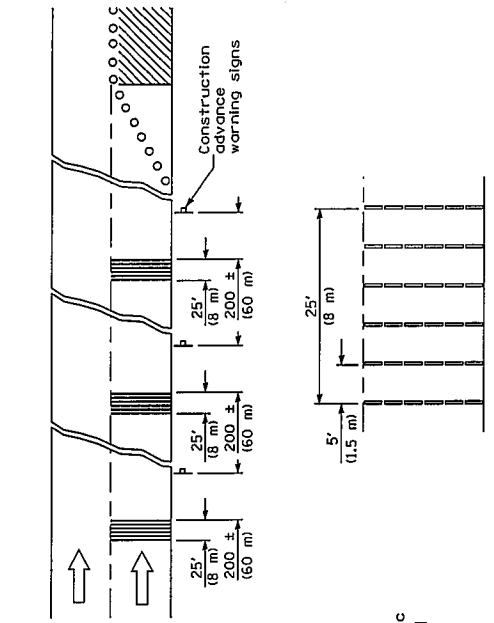
TYPICAL INSTALLATION
