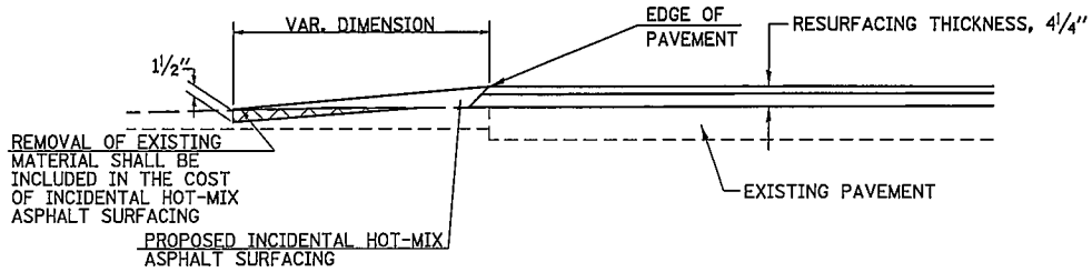
SECTION B-B PROPOSED SIDEROAD TAPER
