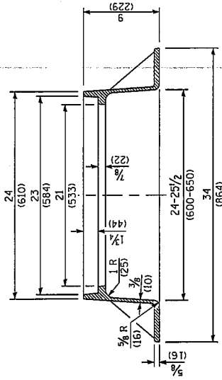
SECTION A-A Gray Iron
